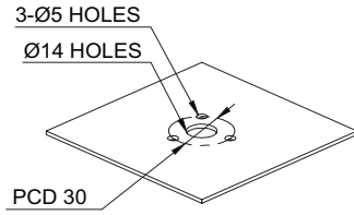
QTC50ML-ETN-BZ
